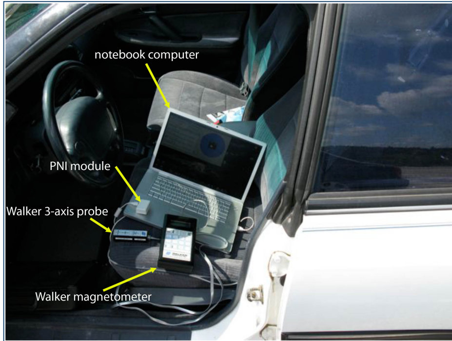
Figure 9 - The driver's seat location of the magnetometers and notebook computer used to record the PNI readings. The PNI module, which we built, consisted of the PNI magnetometer plus a USB interface circuit.
